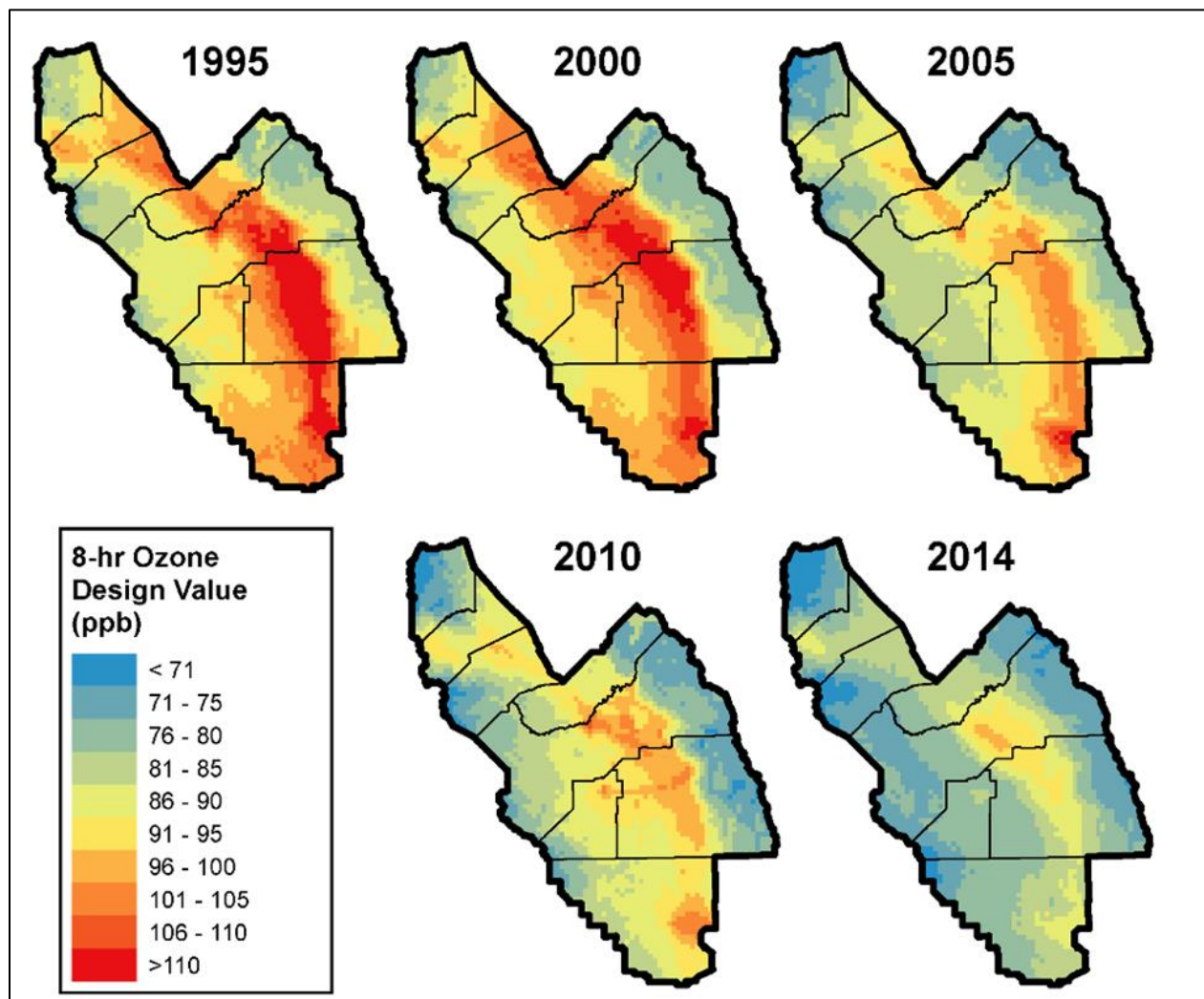
Figure 2-6 Improvement in 8-hour Ozone Design Values, 1995-2014
