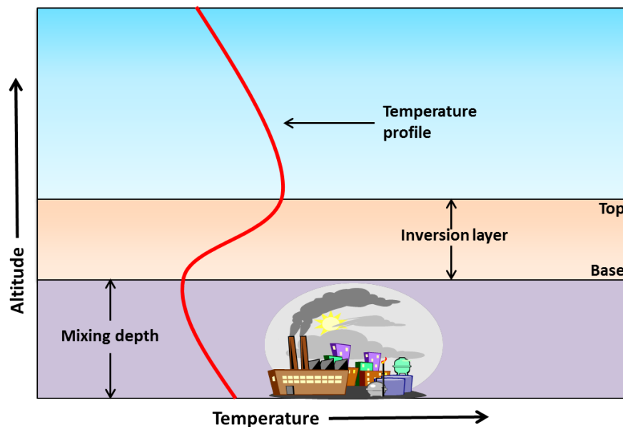
Figure 2-3 Effect of Temperature Inversion on Pollutant Dispersion
