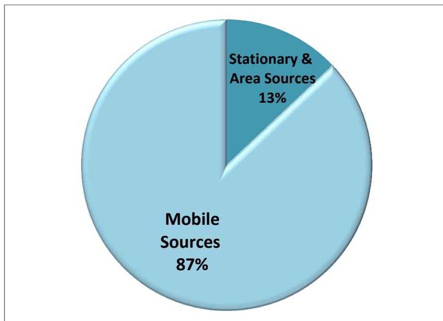
Figure 2-4 Percent Ozone NOx Emissions by Source Type 2
