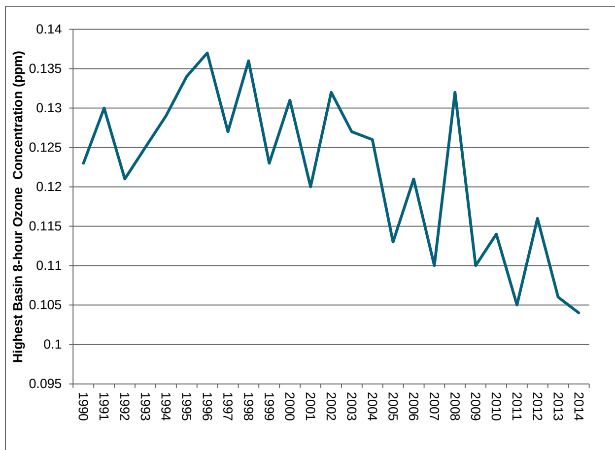
Figure 2-9 Basin Maximum Average 8-Hour Ozone Concentrations
