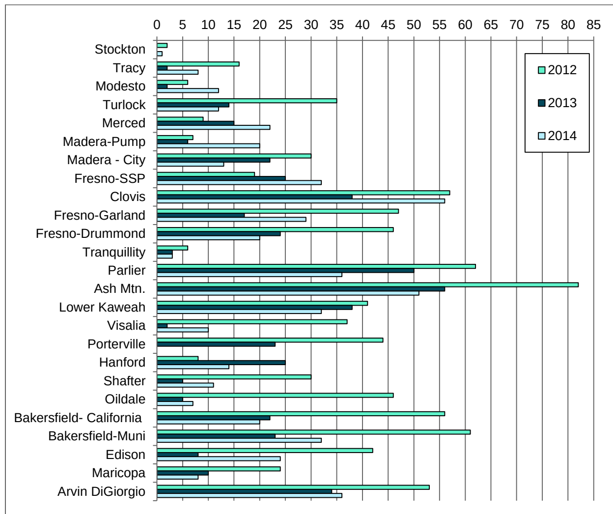
Figure 2-11 Quantity of Days Over the 2008 8-Hour Ozone Standard
