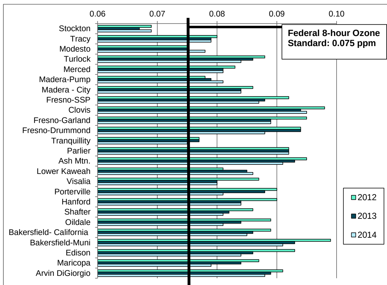
Figure 2-10 8-Hour Ozone Design Values (2012-2014)
