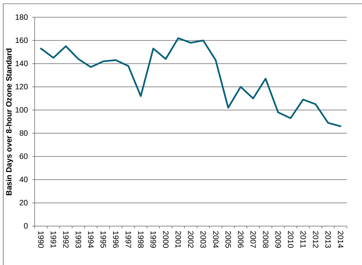
Figure 2-8 Basin Days over the 2008 8-Hour Ozone Standard
