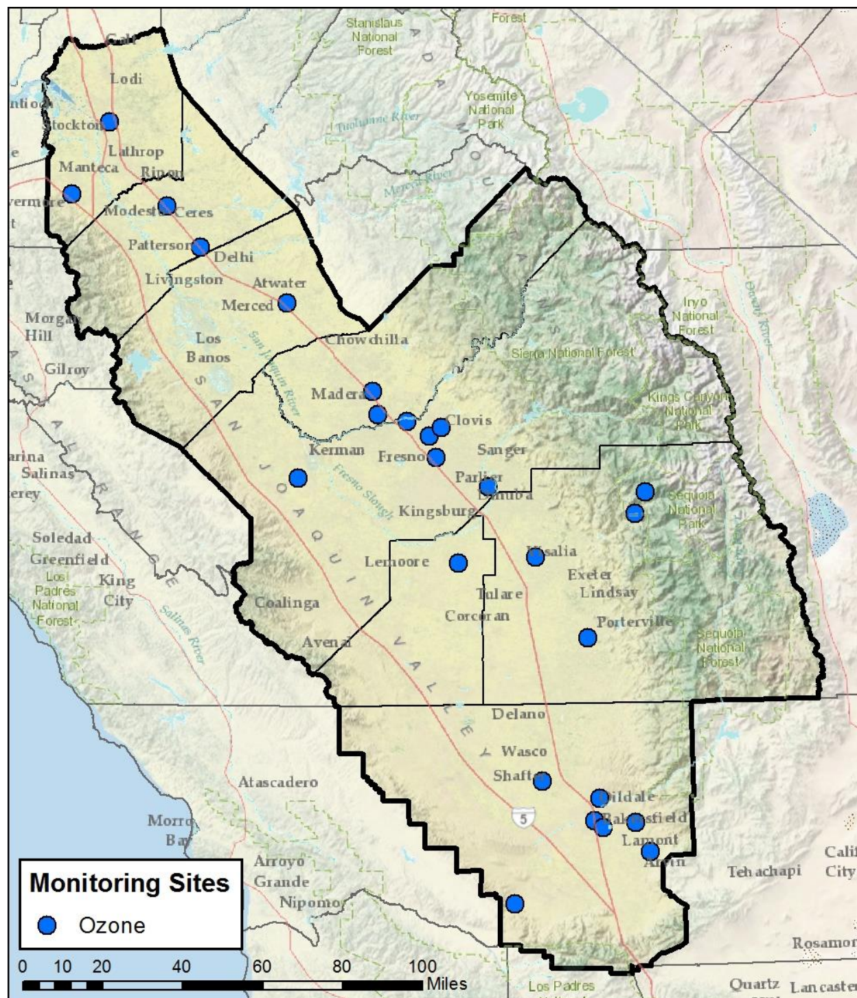
Figure 2-5 Ozone Monitoring Sites within the Valley
