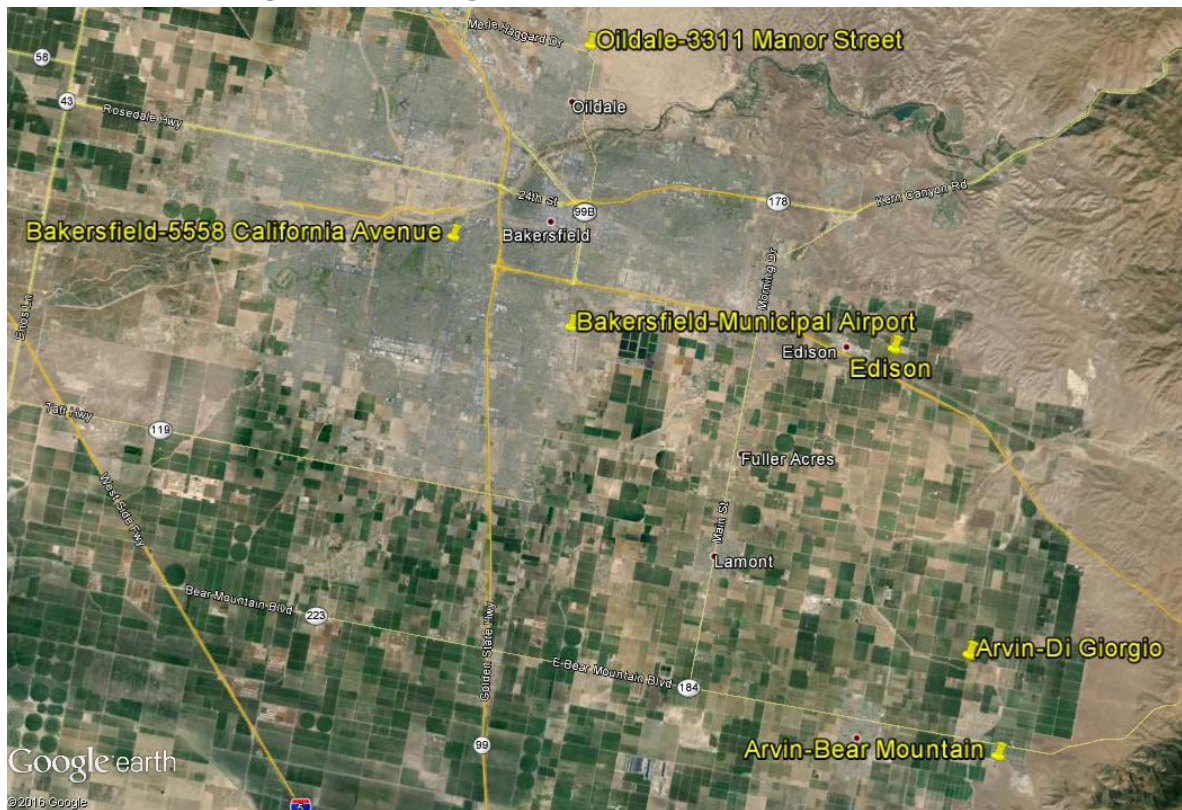
Figure 17. Six High Ozone Sites in the Southern SJV
