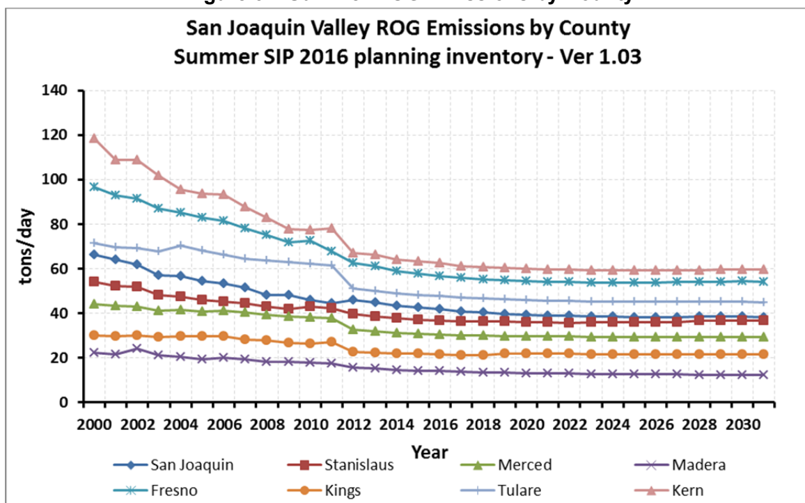
Figure 34. Summer ROG Emissions by County
