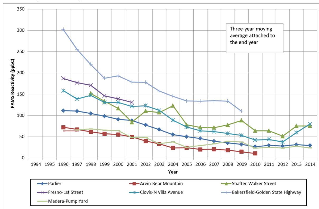
Figure 35. July-August Means at all SJV PAMS Stations (5-7 a.m./6-8 a.m.)*
