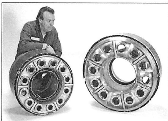
Figure 4. Conventional and SoLoNOx Combustor Liners
