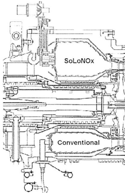
Figure 5. SoLoNOx and Conventional Combustion Systems.
