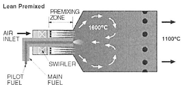
Figure 1. How Lean-Premixed Combustion Reduces NOx Emissions
