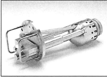
Figure 10b. Titan 250 Fuel Injector
