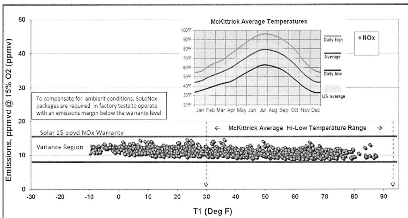
Figure 3. Emission Trends with Variation in Ambient Temperature on Titan 130 SoLoNOx Gas Turbine ( Gas Compression Application in Canada , typically running below full engine load)
