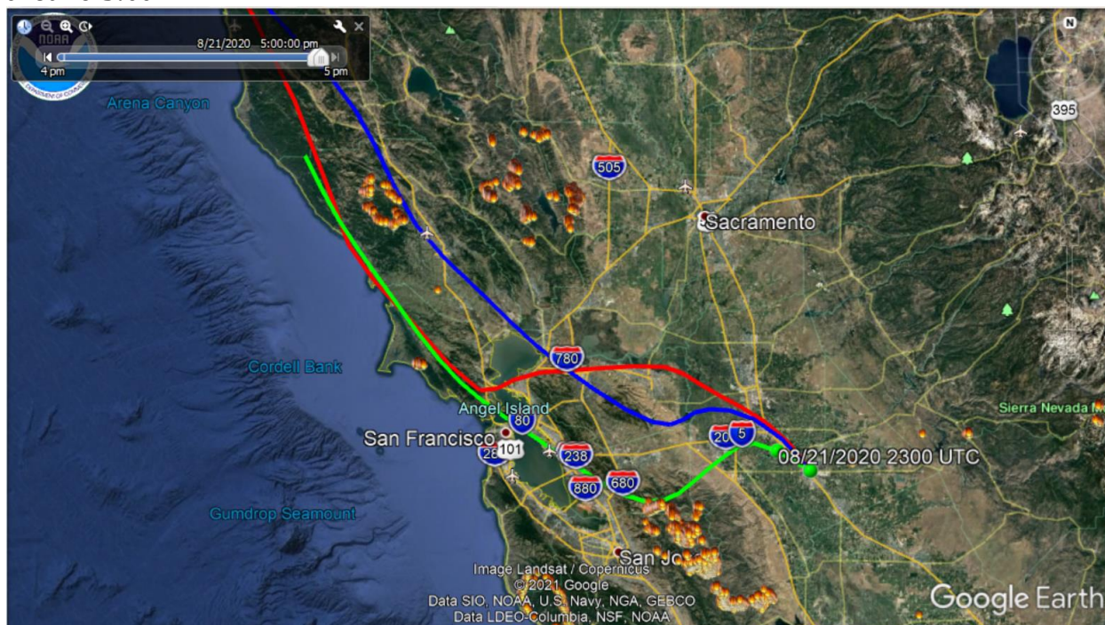
Figure 4-4: Backward Trajectory (24-hour) for August 21, 2020 showing location of air mass arriving in Modesto at 50 (red), 500 (blue), and 1,000 (green) meter height levels around 5:00 PM
