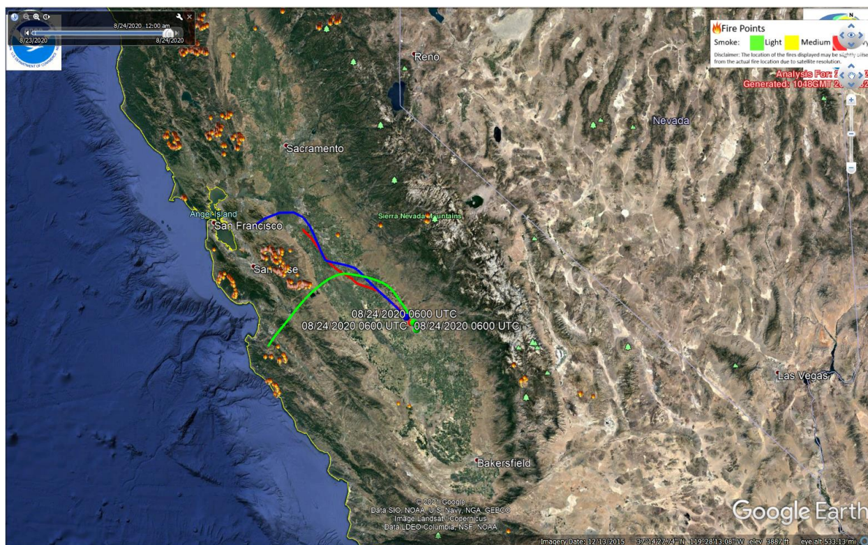
Figure E-16: Backward Trajectory (24-hour) for August 24, 2020, showing location of air mass arriving in Fresno-Foundry at 50 (red), 500 (blue), and 1,000 (green) meter height levels around 12:00 AM.
