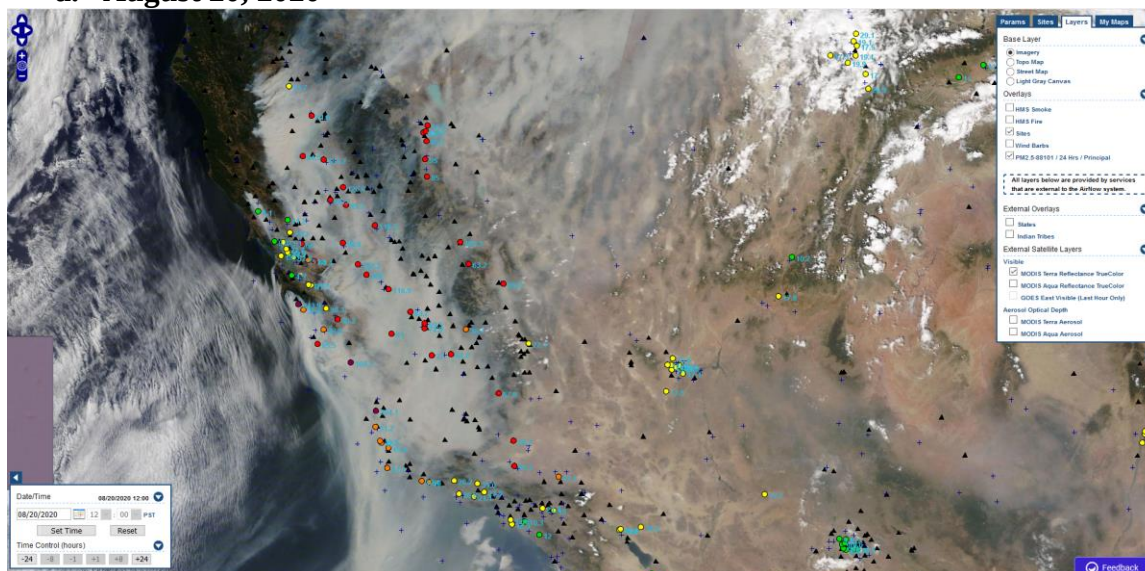
Figure 4-2 (a-e): MODIS Terra Satellite Imagery showing the geographic extent of wildfire smoke on August 20, 2020
