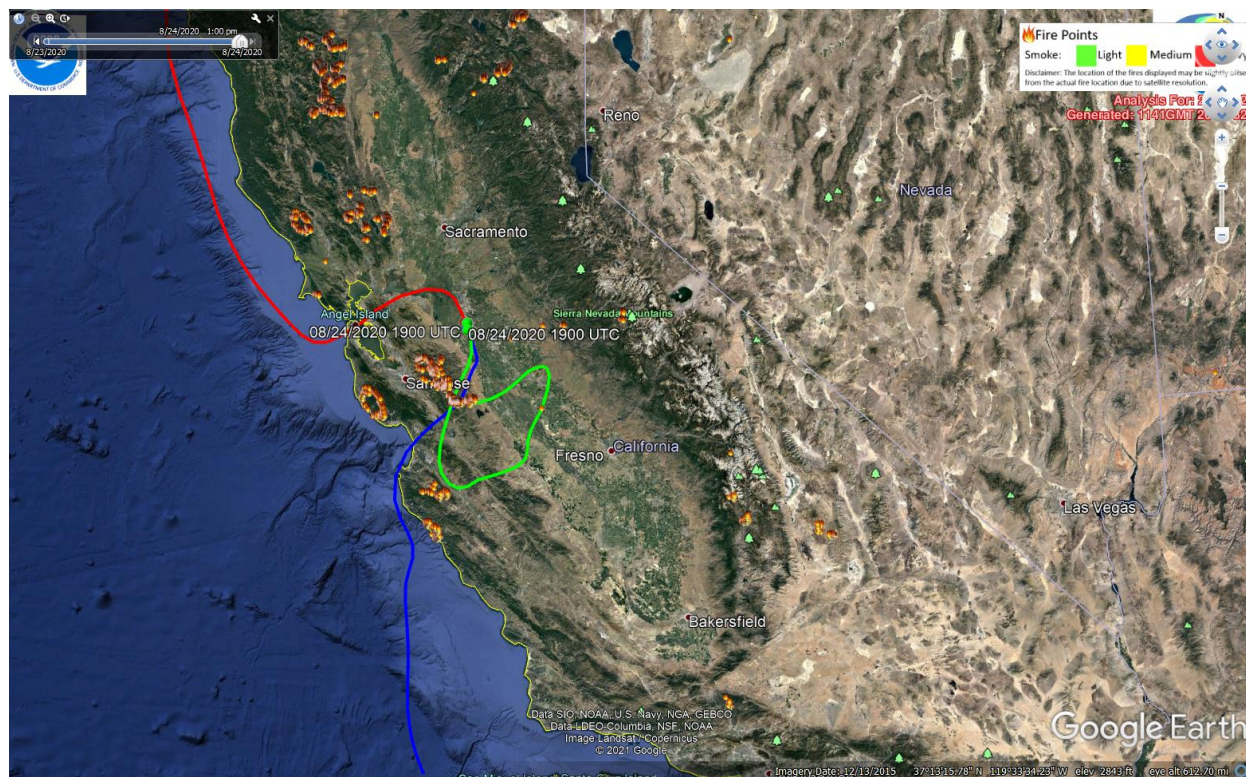
Figure E-7: Backward Trajectory (24-hour) for August 24, 2020, showing location of air mass arriving in Manteca at 50 (red), 500 (blue), and 1,000 (green) meter height levels around 1:00 PM
