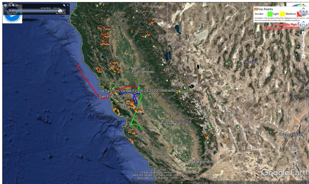
Figure E-3: Backward Trajectory (24-hour) for August 24, 2020, showing location of air mass arriving in Stockton at 50 (red), 500 (blue), and 1,000 (green) meter height levels around 1:00 PM
