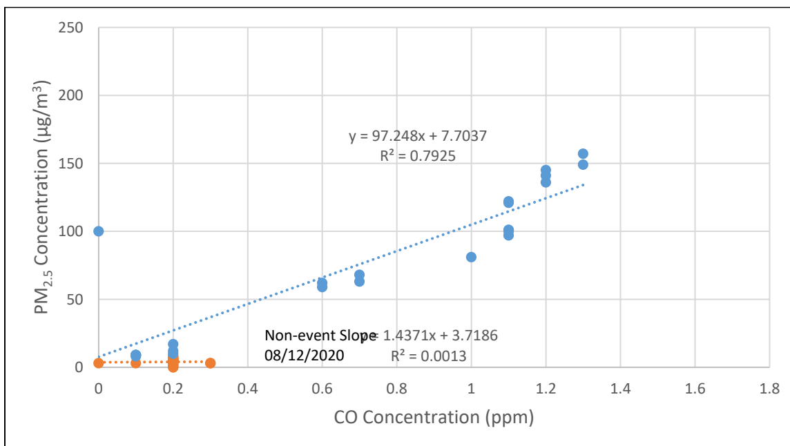
Figure 4-23: Stockton-Hazeltown Hourly PM 2.5 /CO – August 24, 2020
