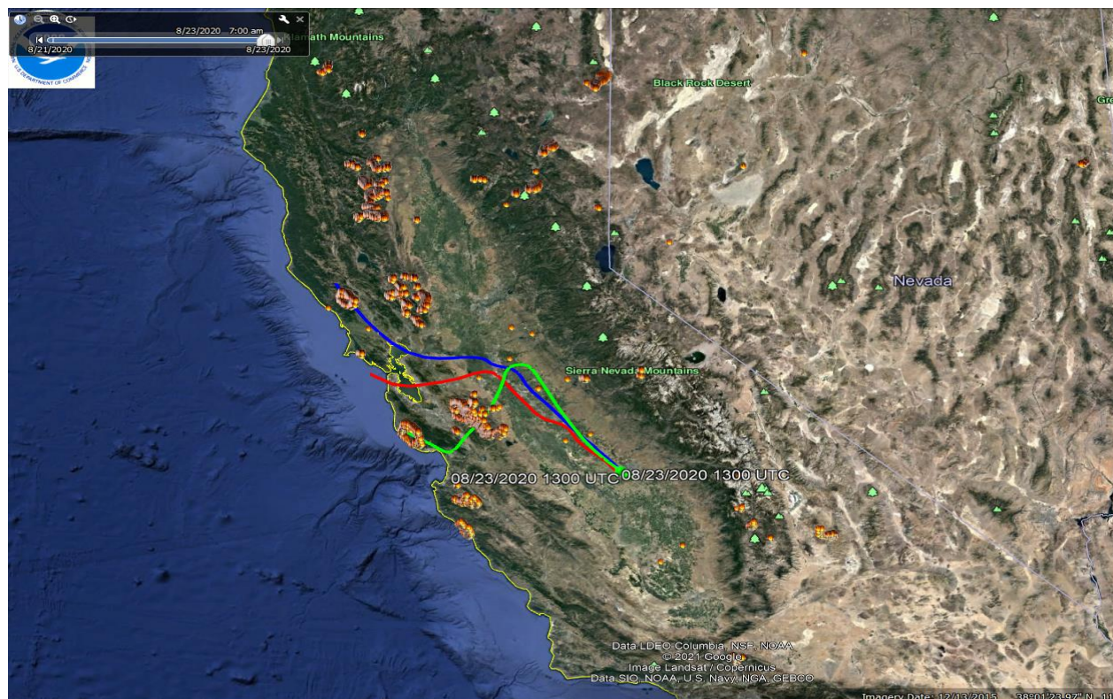
Figure E-15: Backward Trajectory (24-hour) for August 23, 2020, showing location of air mass arriving in Fresno-Foundry at 50 (red), 500 (blue), and 1,000 (green) meter height levels around 7:00 AM.
