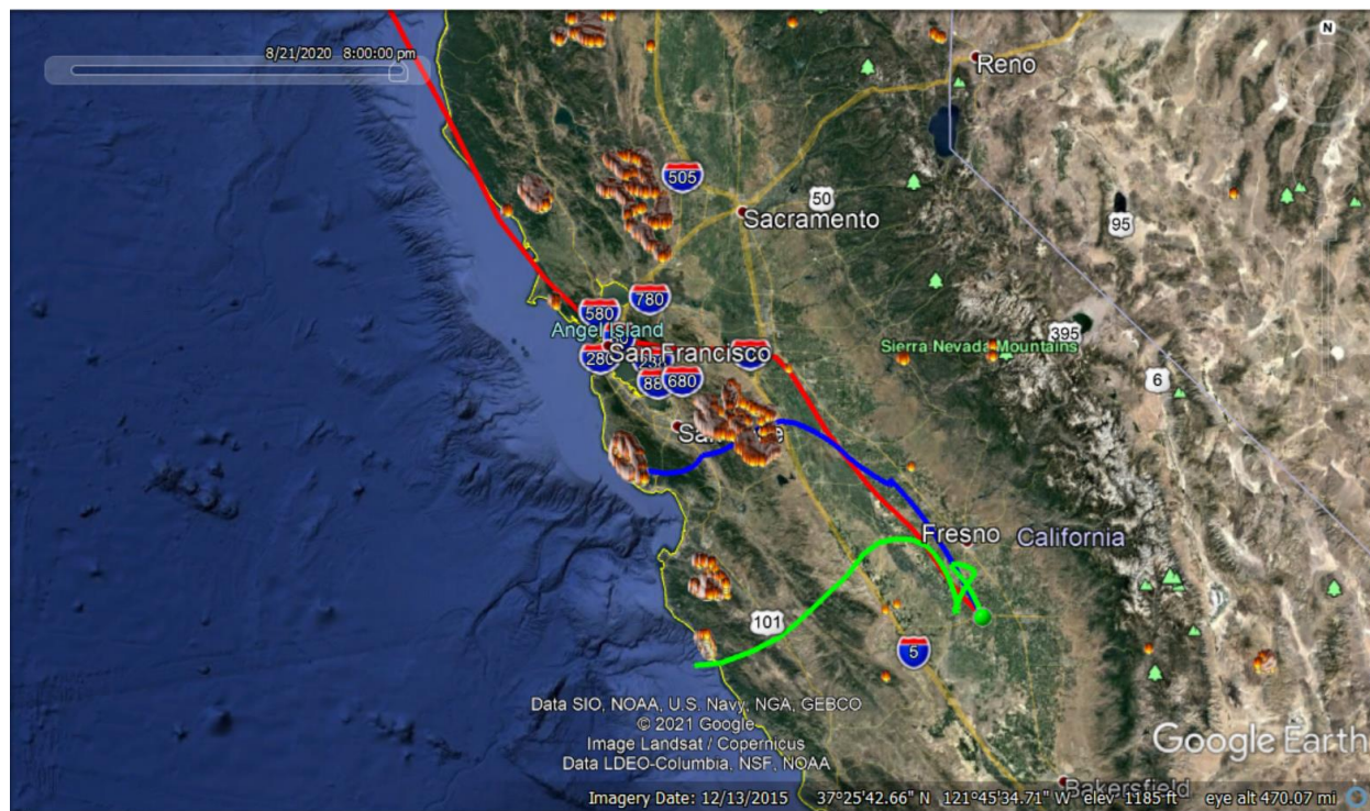
Figure 4-8: Backward Trajectory (36-hour) for August 21, 2020, showing location of air mass arriving in Hanford at 50 (red), 500 (blue), and 1,000 (green) meter height levels around 6:00 PM
