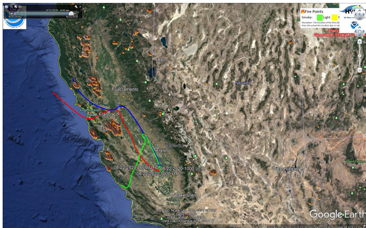
Figure E-18: Backward Trajectory (36-hour) for August 22, 2020, showing location of air mass arriving in Corcoran at 50 (red), 500 (blue), and 1,000 (green) meter height levels around 6:00 AM
