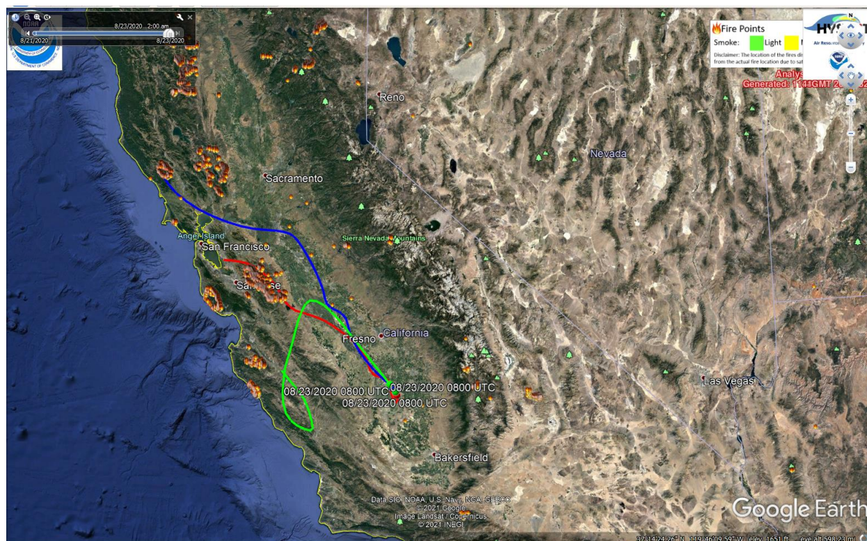
Figure E-19: Backward Trajectory (36-hour) for August 23, 2020, showing location of air mass arriving in Corcoran at 50 (red), 500 (blue), and 1,000 (green) meter height levels around 12:00 AM
