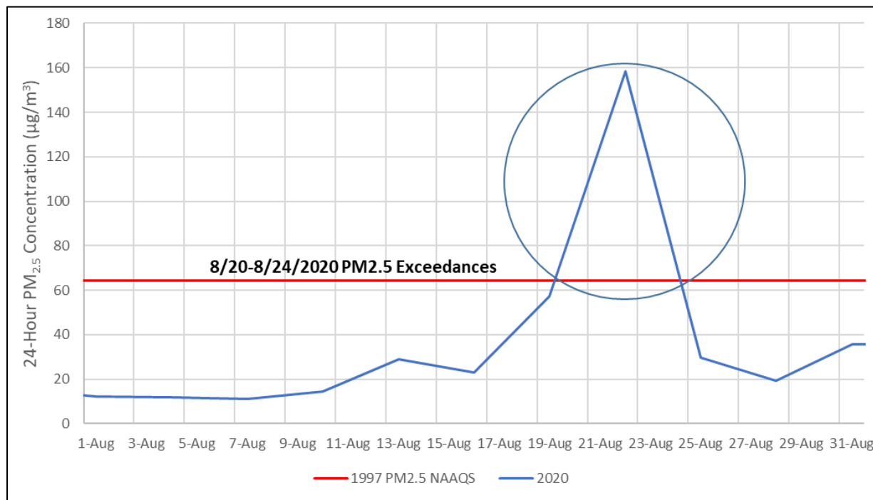
Figure 4-20: Bakersfield-Planiz PM 2.5 Concentrations for August, 2020
