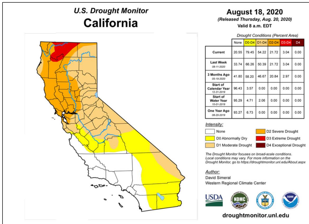
Figure 3-7: Drought conditions that existed across California on August 18, 2020
