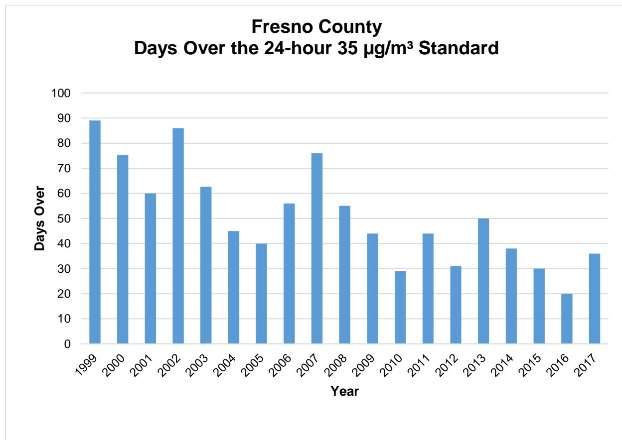
Figure A-31 Fresno County - Days Over the 24-hour 35 µg/m³ Standard 22
