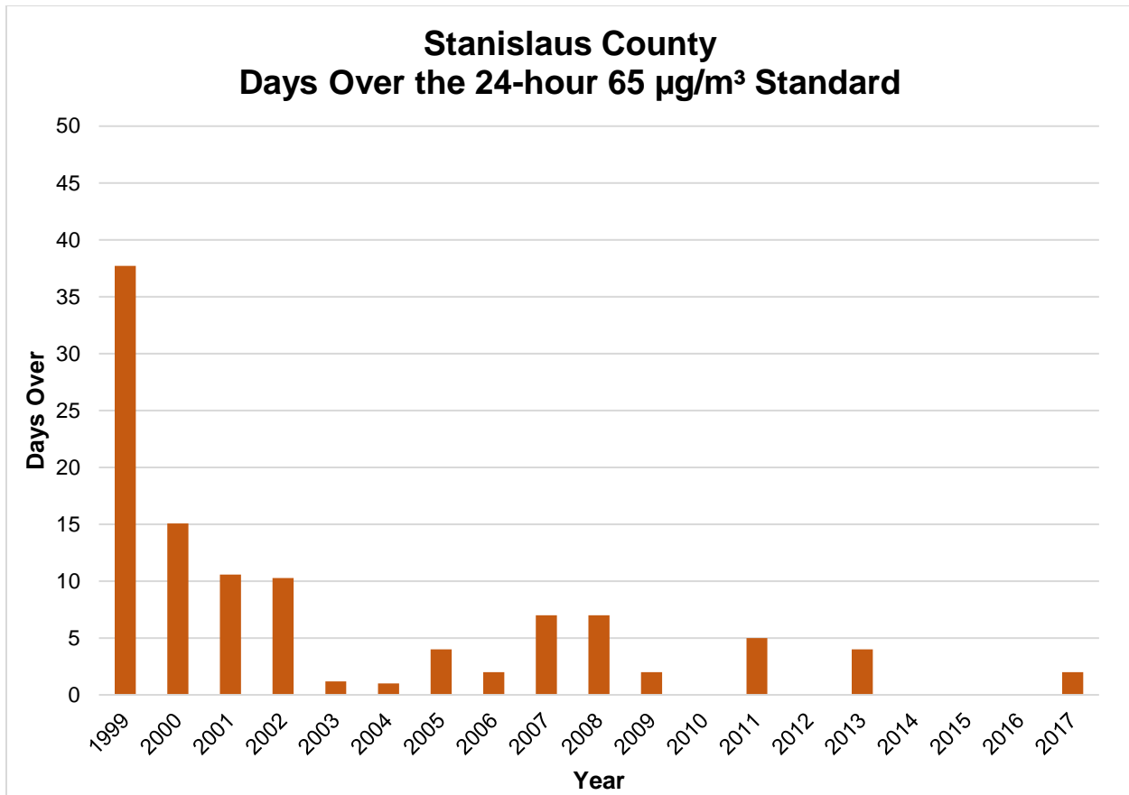
Figure A-20 Stanislaus County – Days Over the 24-hour 65 µg/m³ Standard 9
