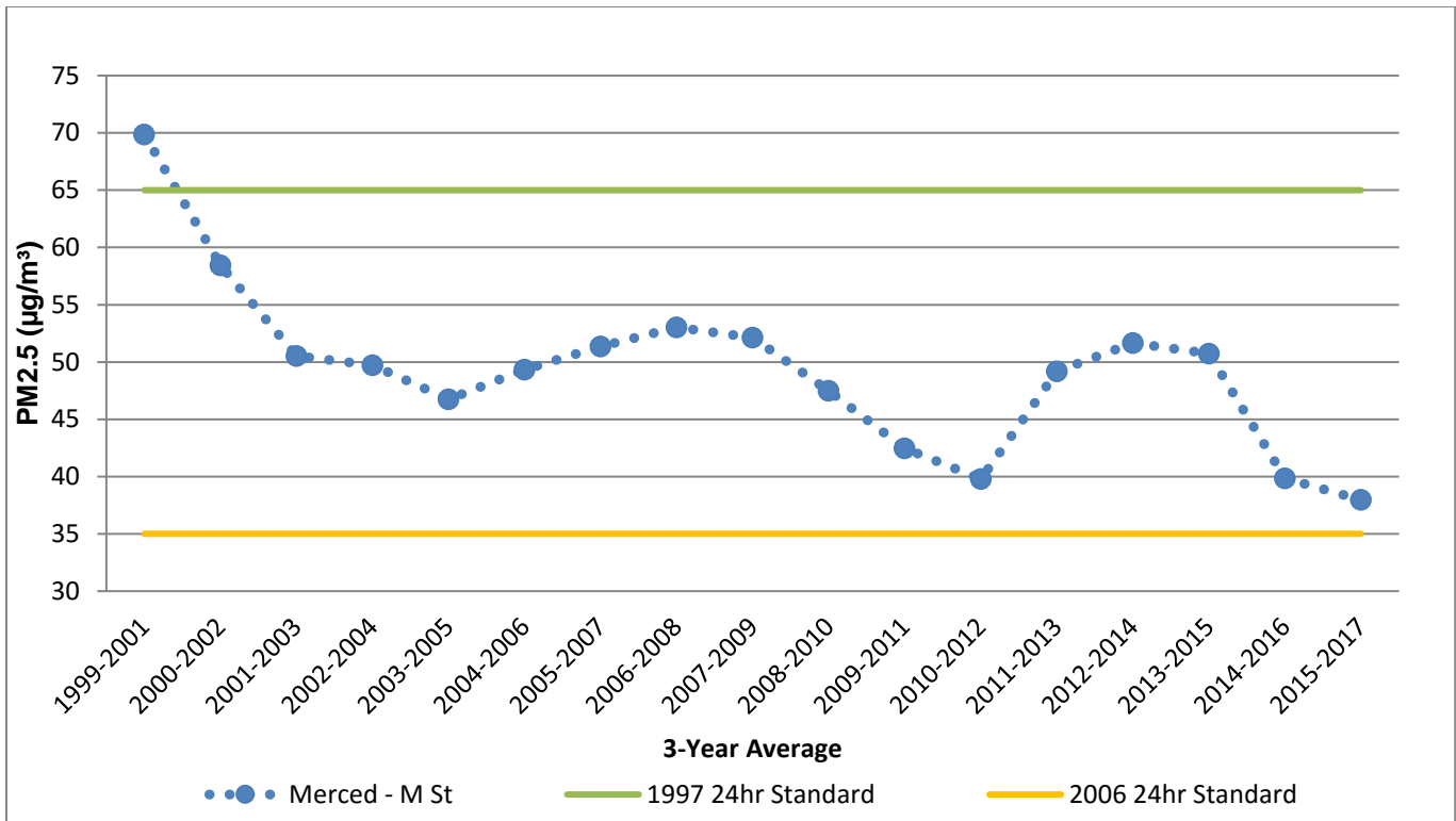
Figure A-8 Merced County Annual Design Value Trend
