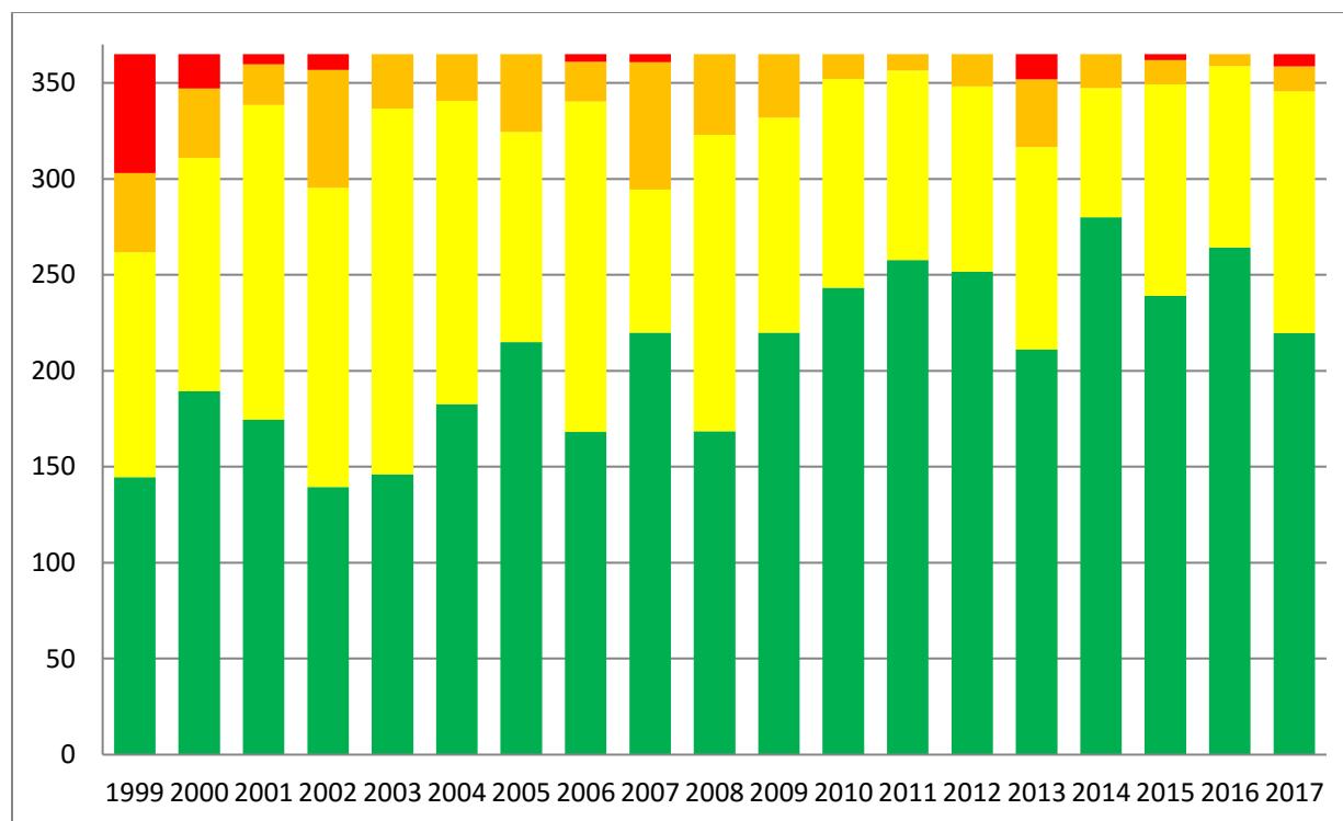
Figure A-39 Madera-City PM2.5 AQI Trend
