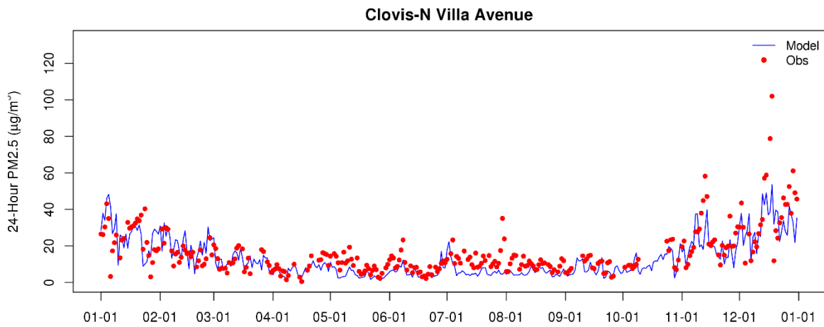
Figure S. 42 Observed and modeled 24-hour average PM 2.5 at Clovis – Villa Avenue
