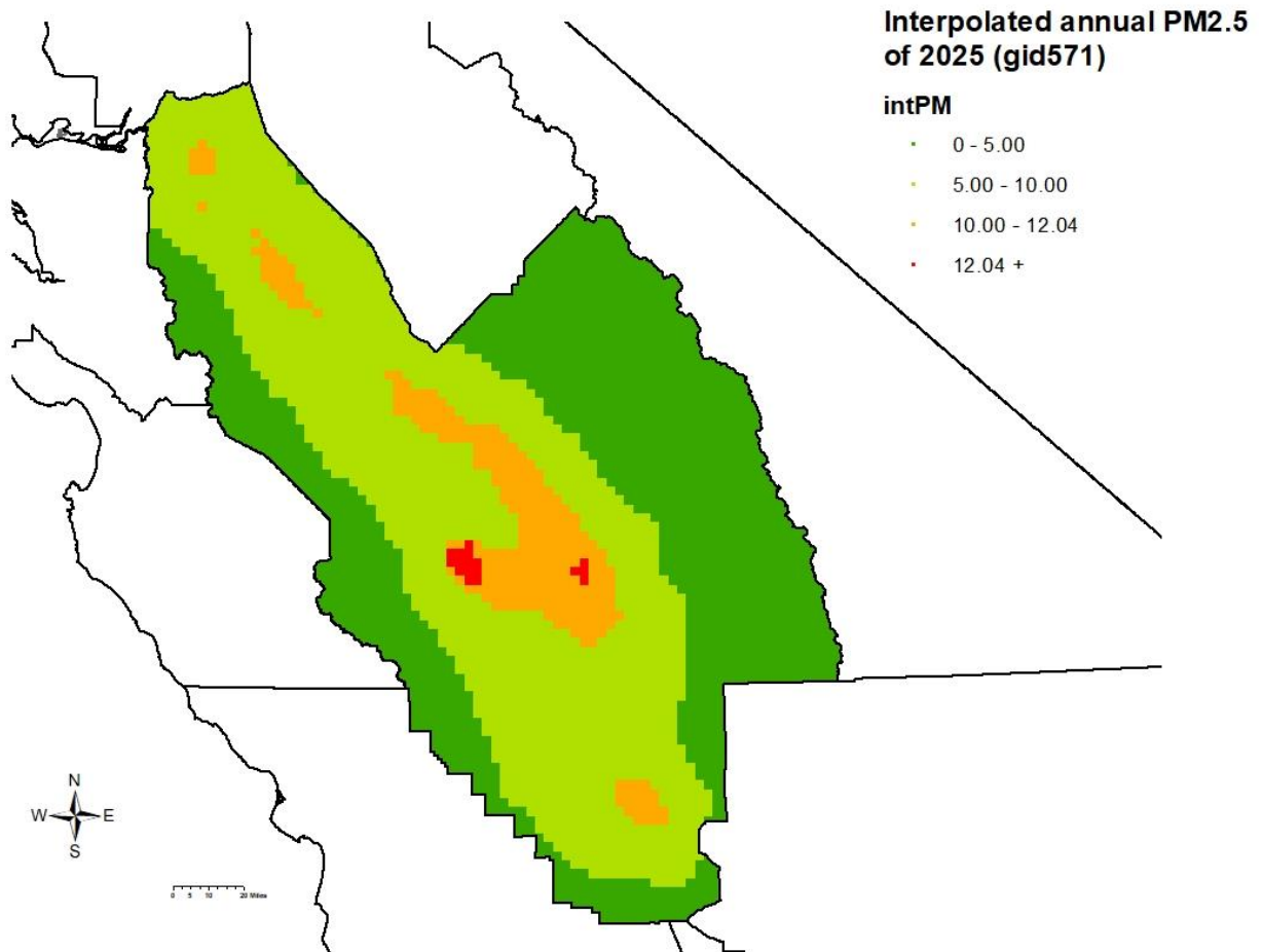
Figure 18. Spatial distribution of projected 2025 annual PM 2.5 DVs within the SJV nonattainment area. All grid cells have DVs not greater than 12.04 µg/m 3 except for a few cells surrounding the Lemoore Naval facility and Visalia.
